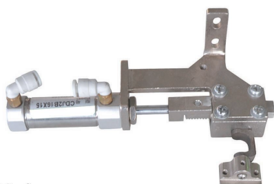
Flip flop
